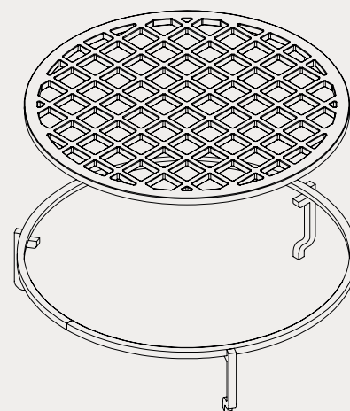
Two-piece grate; grill and frame
